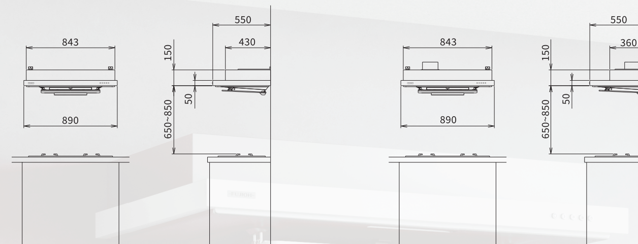
FR-FS2290VP (Ventilating) [mm]
